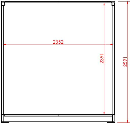
40ft Shipping Container - Section
