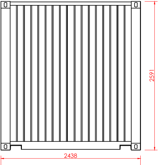
40ft Shipping Container - Front Elevation
