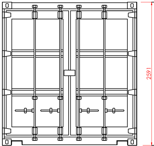
40ft Shipping Container - Door Elevation
